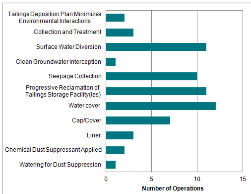
Figure 6-12: Techniques Employed to Minimize Tailings-Environment-Water Interactions (18 Operations)
