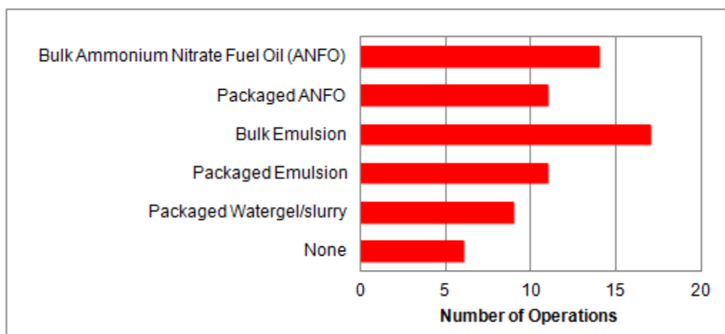
Figure 6-7: Relative Use of Types of Explosives at Base Metal Operations (29 Operations)
