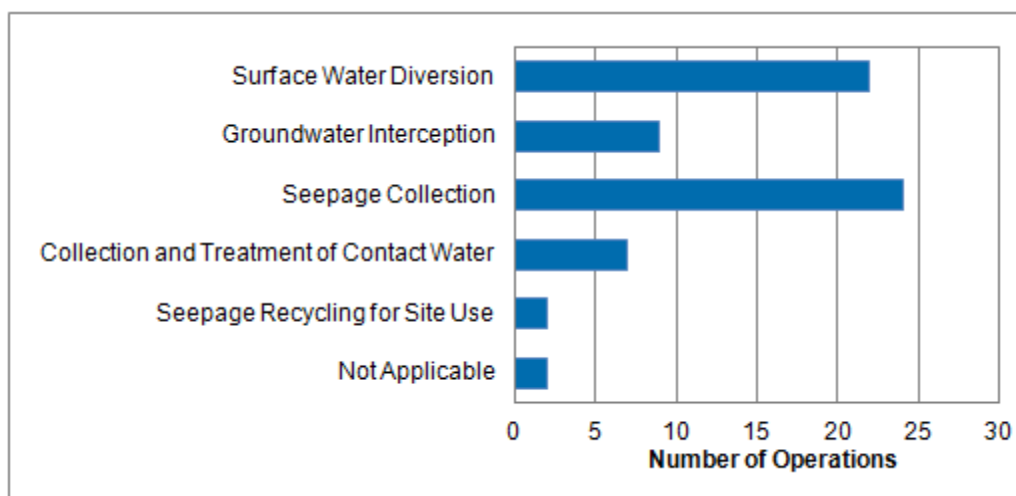
Figure 6-6: Base Metal Subsector Mine-Water-Environment Interaction Minimization Techniques (31 Operations)
