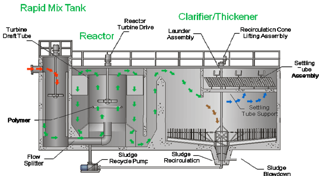
Figure 8-8: DensaDeg® Process
