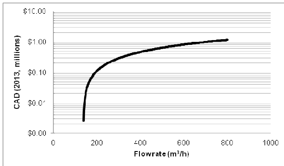
Figure 8-6: Media Filtration Equipment Costs
