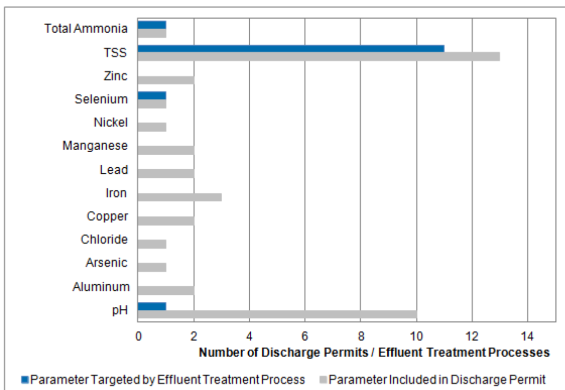
Figure 6-61: Parameters Included in Discharge Permits and Targeted by Effluent Treatment Processes at Reviewed Coal Operations (15 Operations Discharge Permits / 11 Operations Effluent Treatment Processes)
