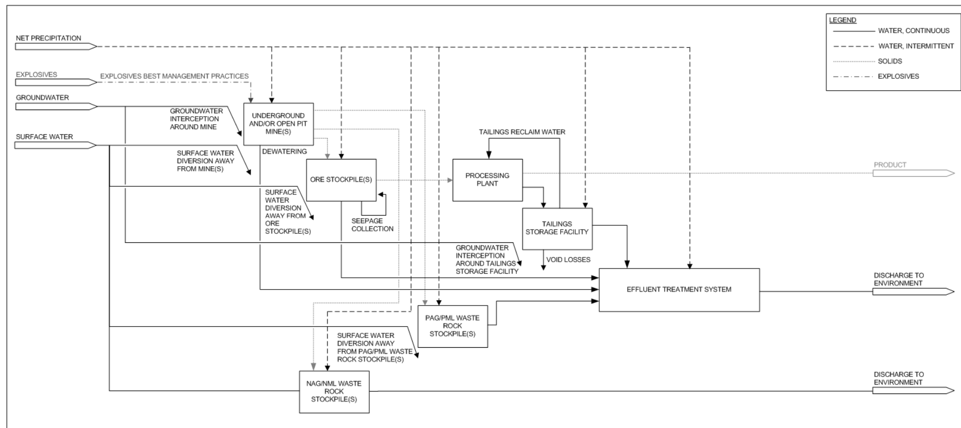
Figure 6-58: Diamond Sector Water Management Model
