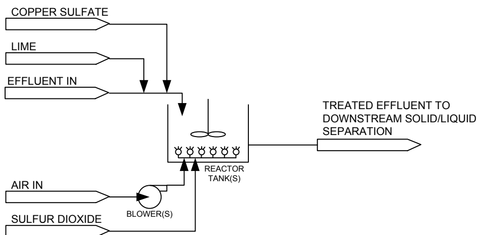
Figure 8-10: Simplified INCO \text{SO}_2 /Air Cyanide Destruction Process Flow Diagram
