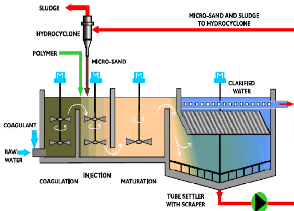
Figure 8-7: ACTIFLO® Process
